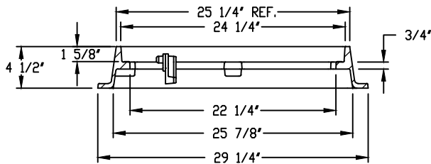
FRAME SECTION B-B
