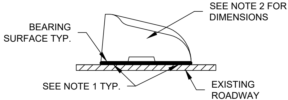
SECTION - SLOPED
